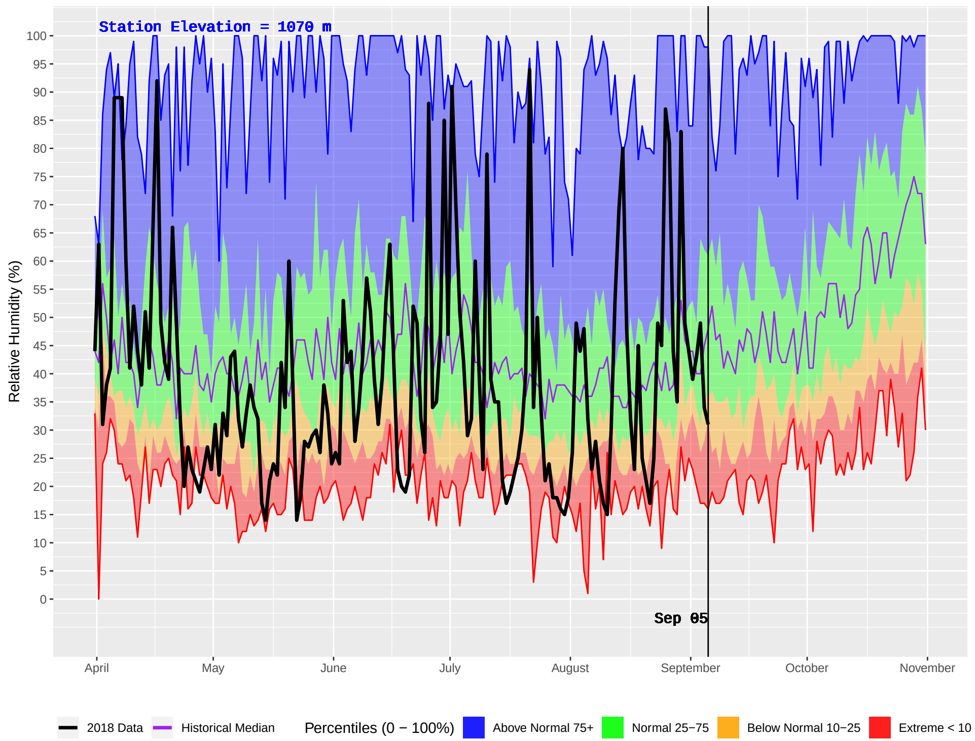
MEADOW LAKE (236) : Historical (1991–2016) and Current (2018) Daily Relative Humidity
